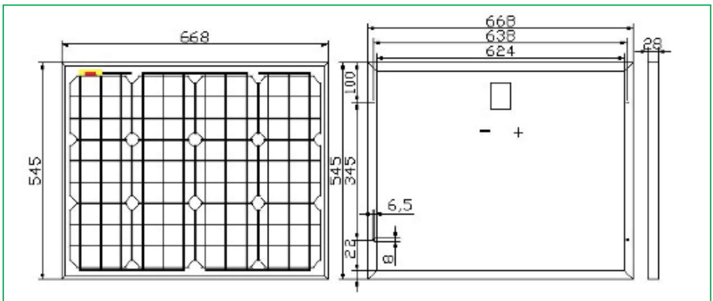
PV Drawing
